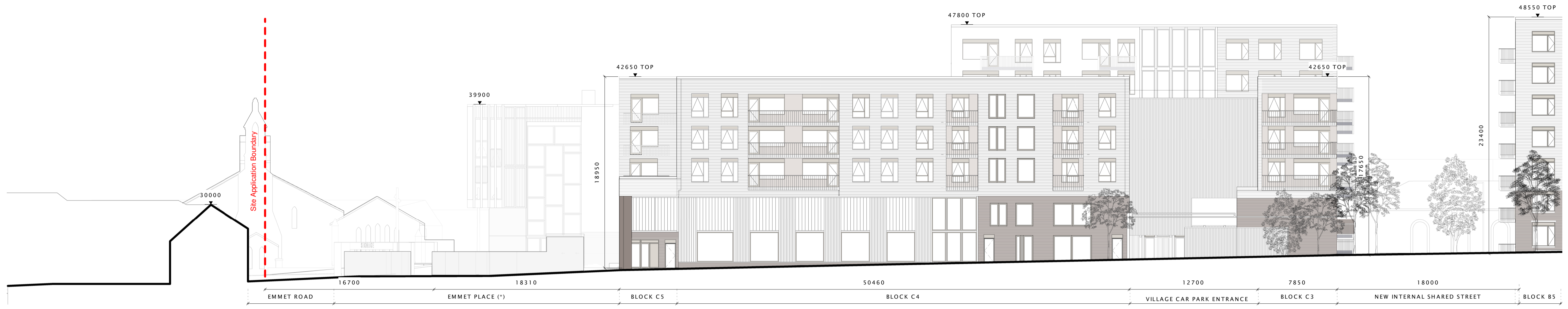
1 CONTEXTUAL ELEVATION - WEST (ST. VINCENT STREET WEST) 1/3
